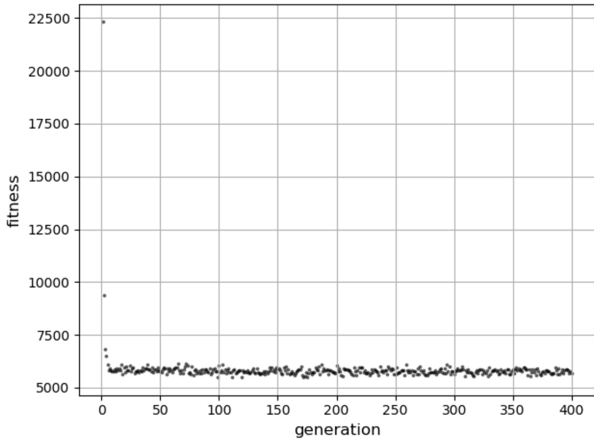
Fig. S1 A convergence plot demonstrating the performance of the GA algorithm over its runtime.
