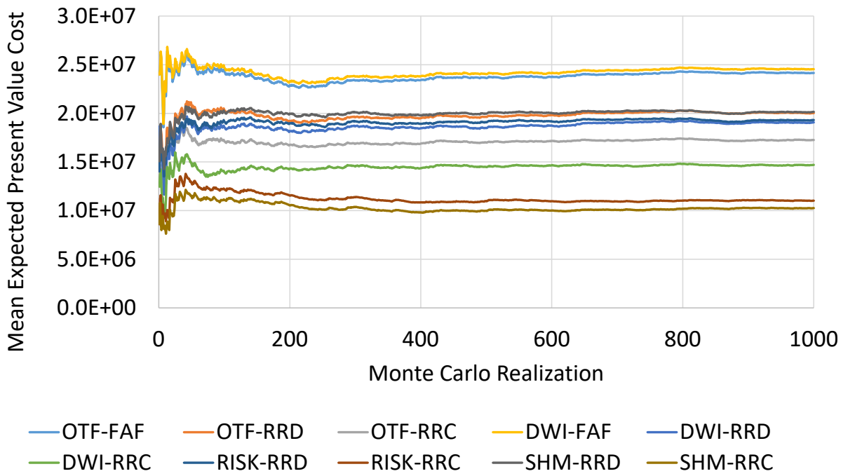
Convergence of the Mean
