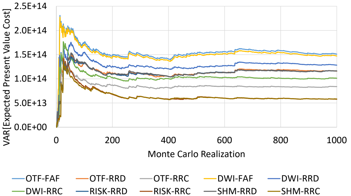
Convergence of the Variance
