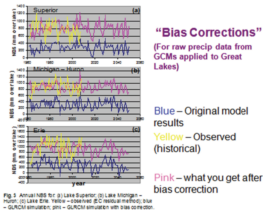
Figure A.2. Annual Net Basin Supply for (a) Lake Superior; (b) Lake Michigan – Huron; and (c) Lake Erie. Yellow – observed (EC residual method); blue – Great Lakes Regional Climate Model (GLRCM) simulation; pink – GLRCM simulation with bias correction.
