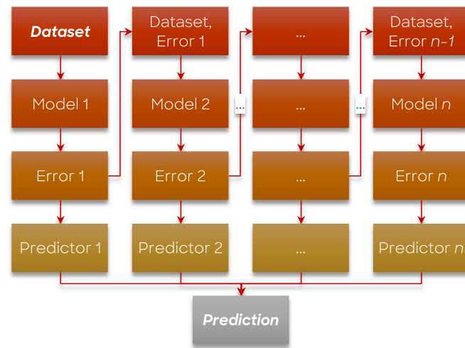
Fig. 6. Boosting approach.
