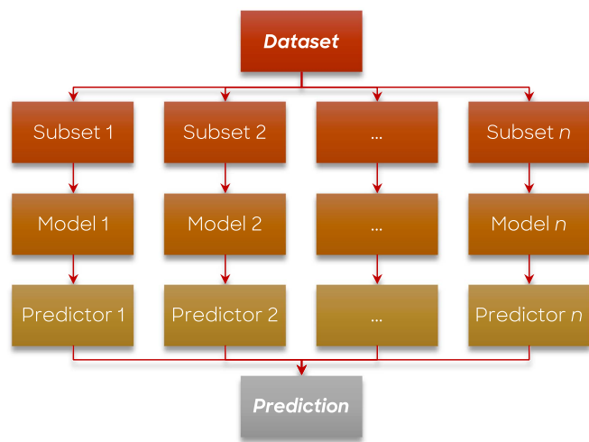
Fig. 5. Bagging approach.
